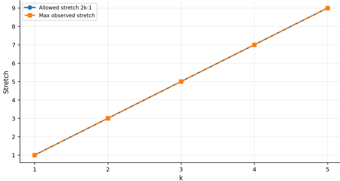
Figure 2. Maximum observed stretch compared with the theoretical bound 2k-1 .
