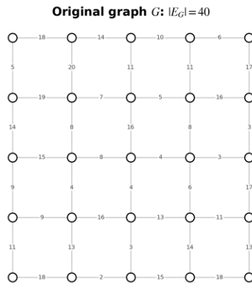
Figure 6. Weighted planar grid: 40 original edges reduced to 24 spanner edges at k=3 .
