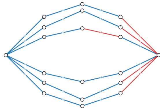
Greedy spanner H_k: |E_H|=24, \max d_H/d_G=1.00
