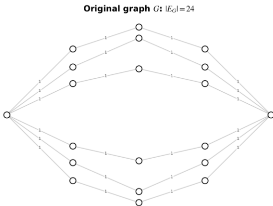
Figure 7. Theta-style example: no edge reduction at the matching target k=3 , illustrating a hard family.
