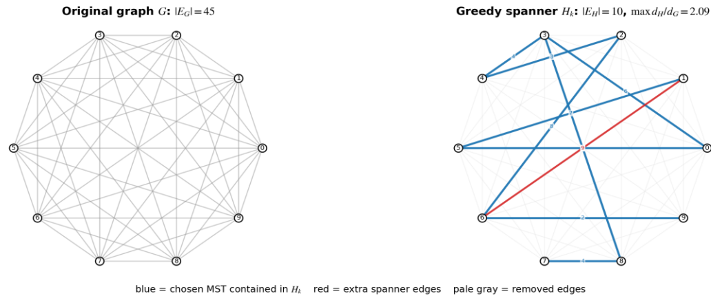
Figure 5. Complete weighted graph: 45 original edges reduced to 10 spanner edges at k=2 .
